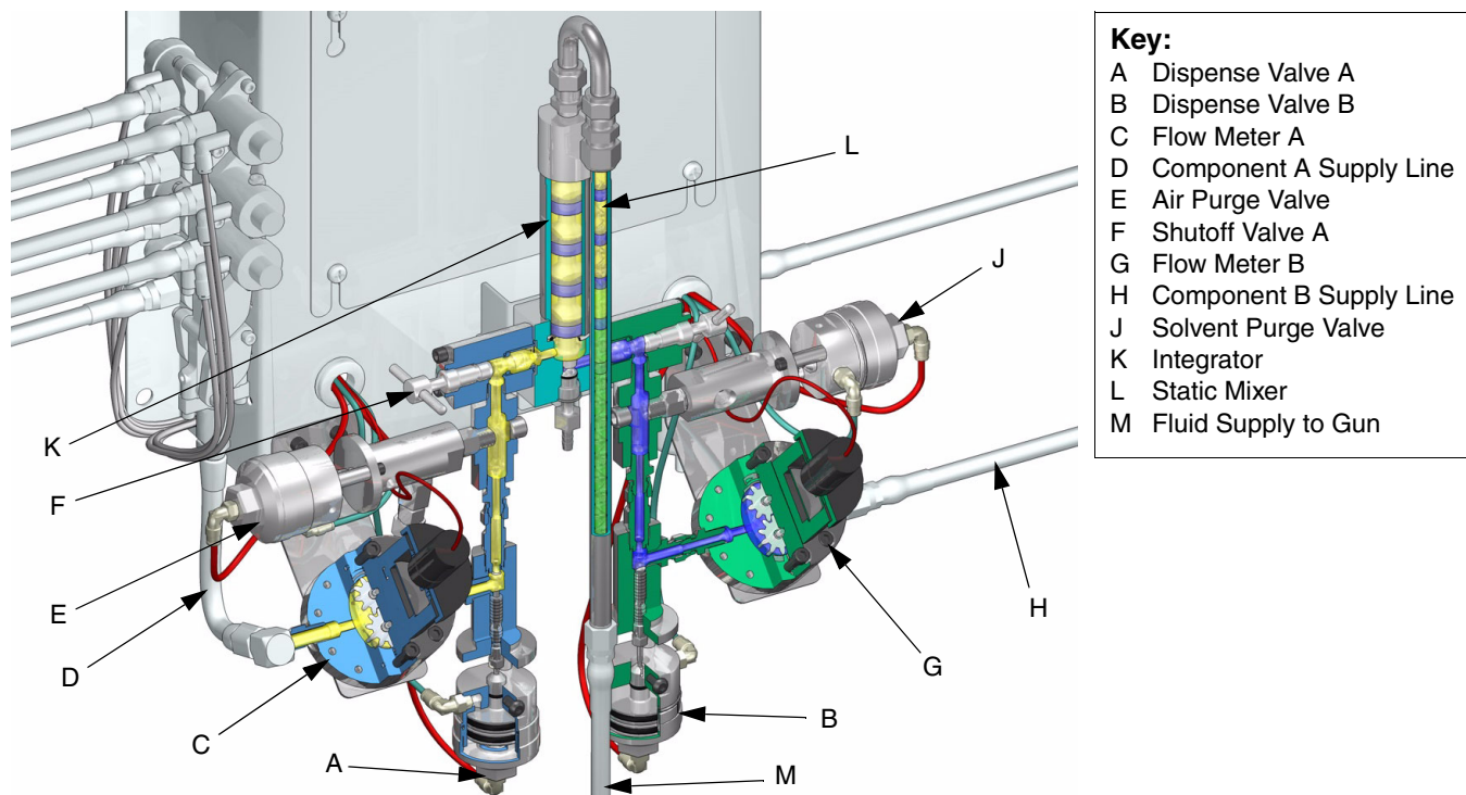
FIG. 2 Fluid Manifold Cutaway
