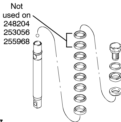
Fig. 7. Remove packings and glands from piston rod.
